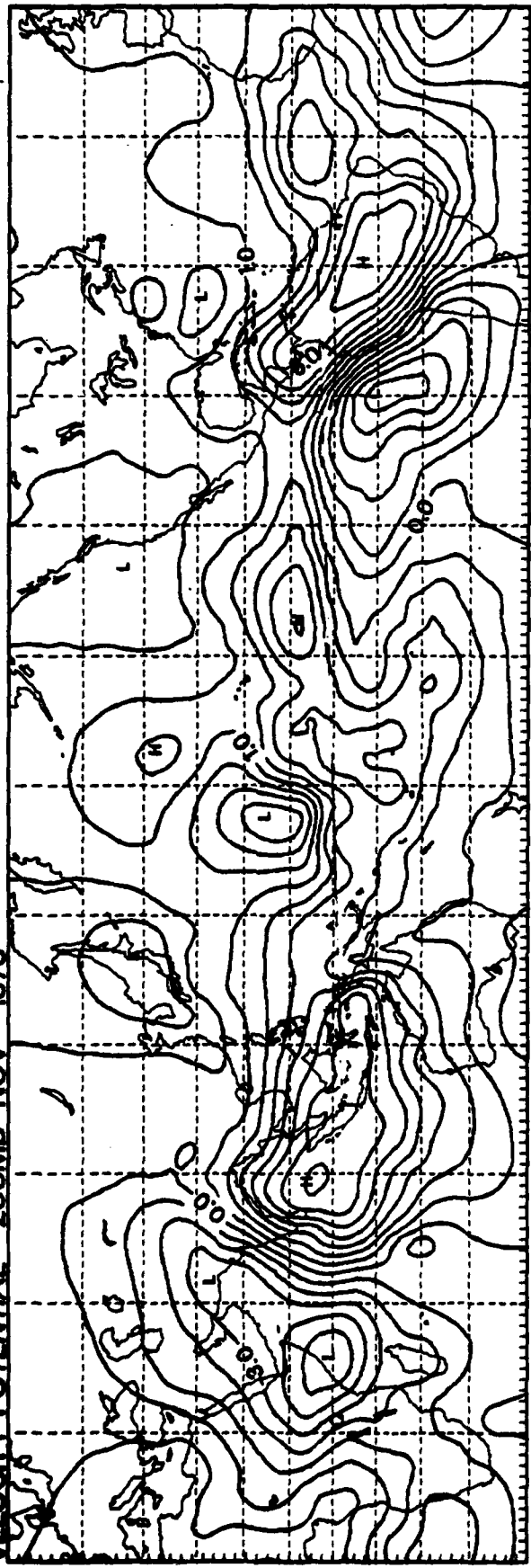
VELOCITY POTENTIAL 200MB NOV 1975
